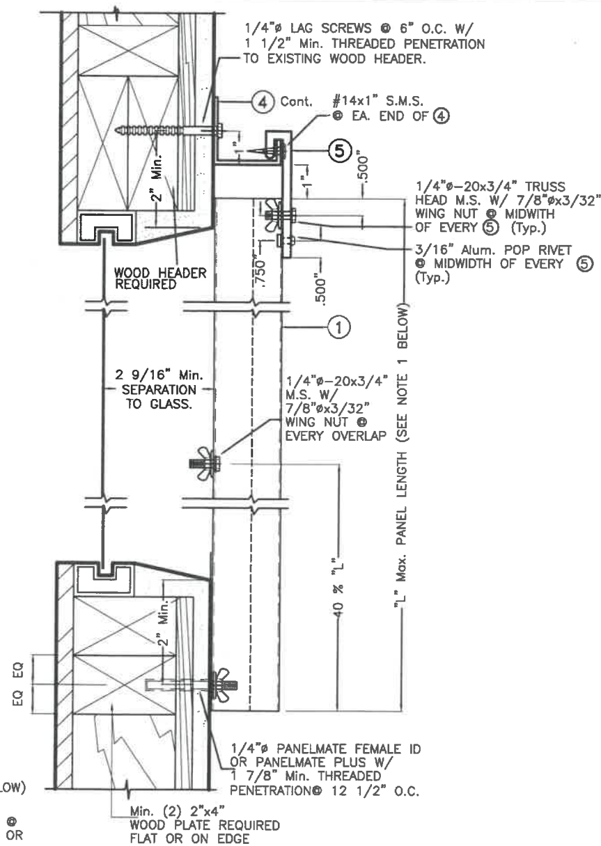
WALL MOUNTING INSTALLATION ALTERNATIVE 2'W SCALE 1/4"=1"
