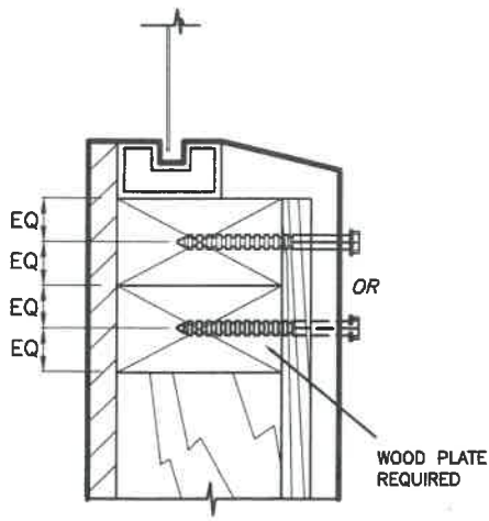
ALTERNATIVE 1W SCALE 3/8=1"
