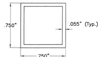
⑧ STOP BAR 11" LONG 6063-T5 Alum. ALLOY
