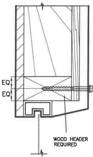
ALTERNATIVE 2W SCALE 3/8=1"
