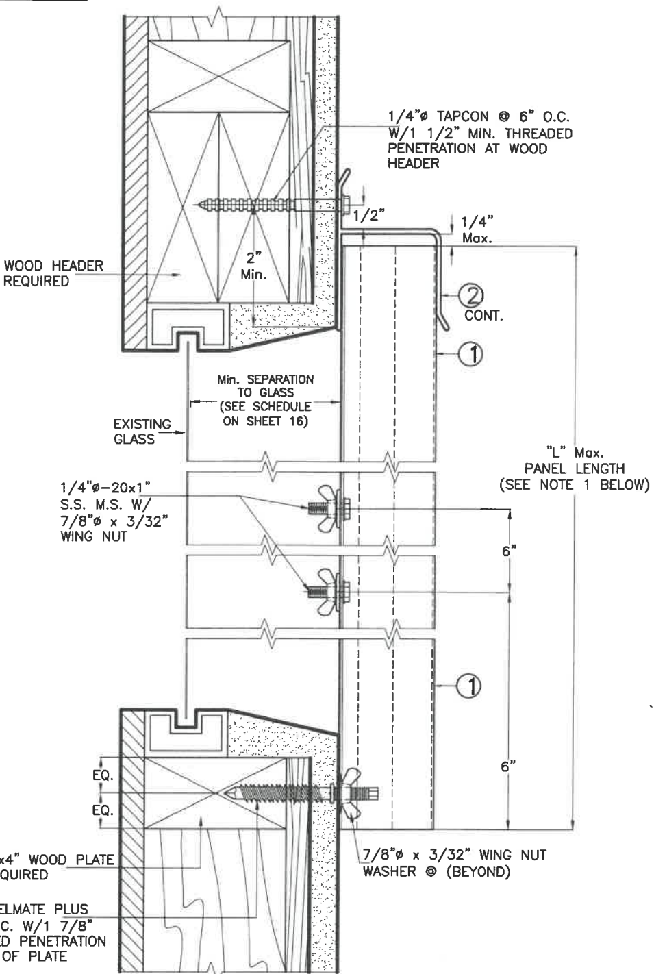
WALL MOUNTING INSTALLATION ALTERNATIVE 8BW ● LIFE SAFETY PANEL
