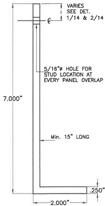
8 2"x7"x1/4" ALUMINUM ANGLE
