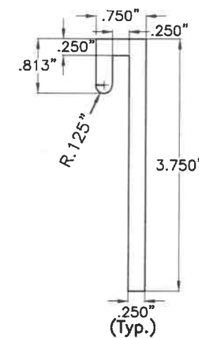
⑤ PANEL HANGER 1 1/4" WIDE 6061-T6 Alum. ALLOY
