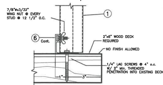
FLOOR MOUNTING INSTALLATION - SECTION 4AW SCALE: 1/4" = 1"
