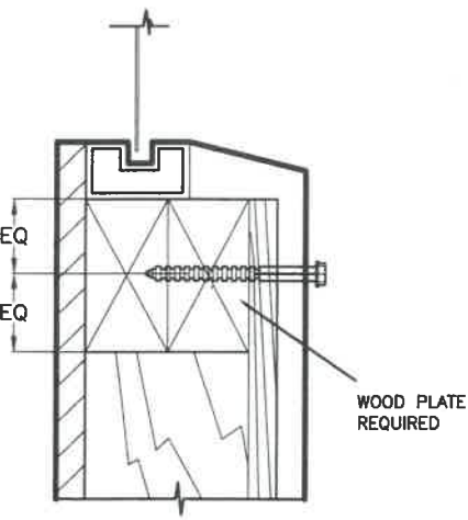
ALTERNATIVE 2W SCALE 3/8=1"
