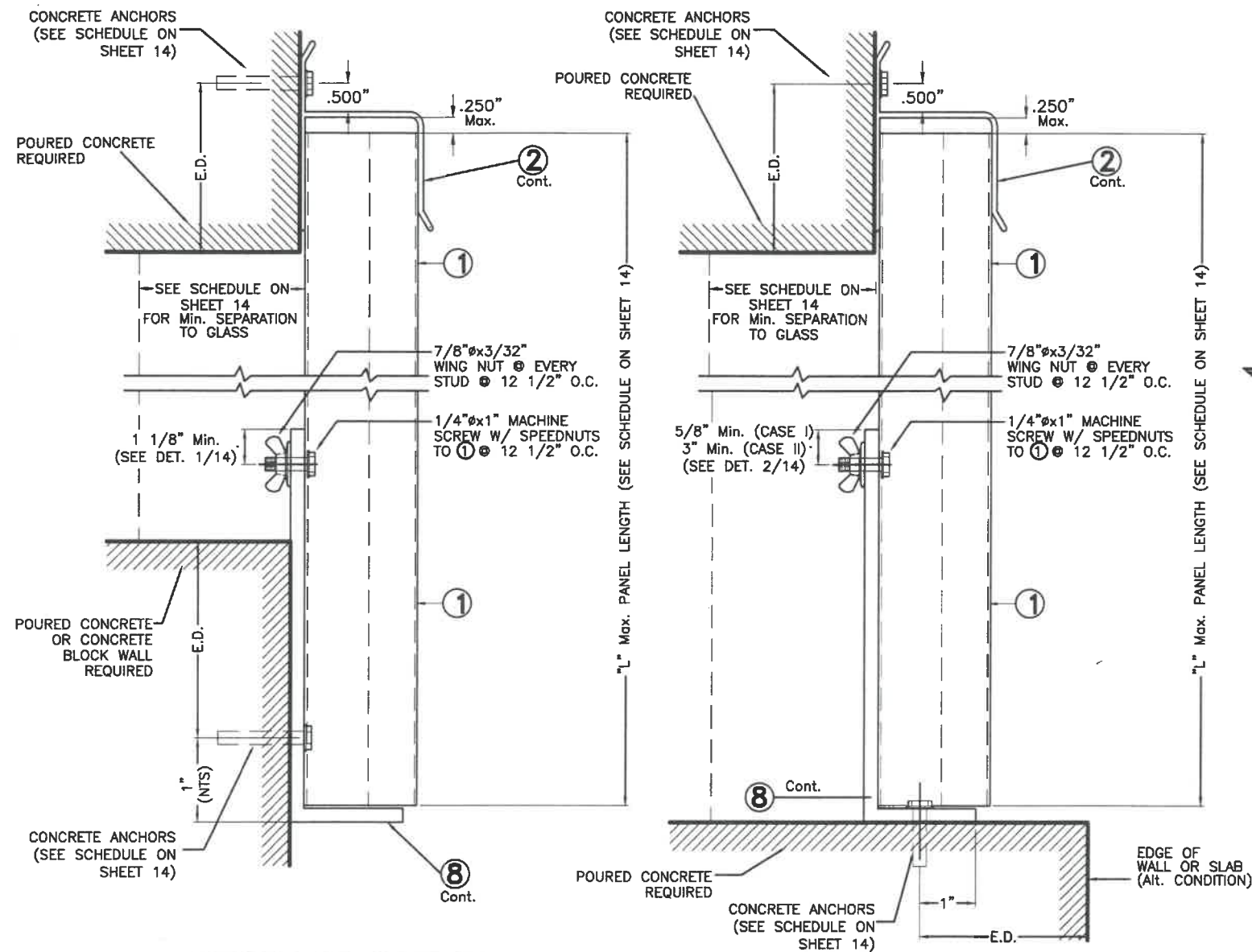
WALL MOUNTING INSTALLATION - SECTION 1 SCALE: 3/8" = 1"
