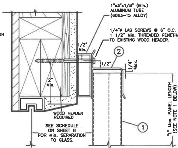
WALL MOUNTING INSTALLATION - ALTERNATIVE 3W SCALE: 1/4" = 1"
