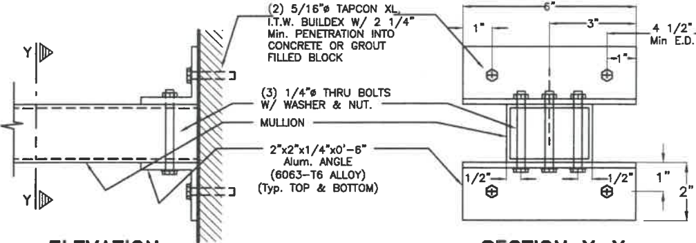
ELEVATION SCALE 1/4"=1"
