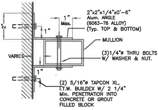
SECTION X-X SCALE: 1/4" = 1"
