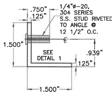
4A ANGLE WITH STUD
