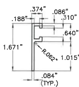
6A 3/8" "F" TRACK
