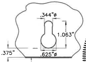
5A KEY HOLE AT PANEL
