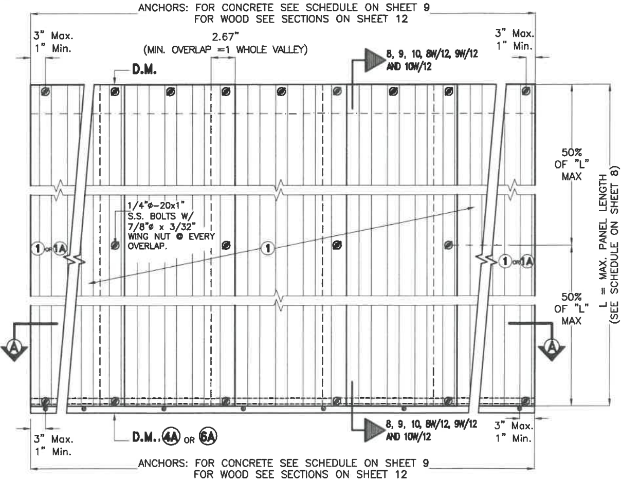
REGULAR STORM PANELS ① & 1A ELEVATION SCALE 3/32"=1"
