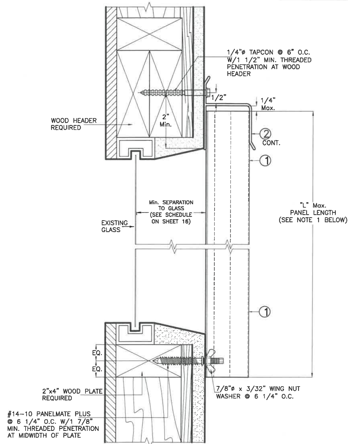
WALL MOUNTING INSTALLATION ALTERNATIVE 8AW ● REGULAR PANEL
