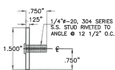
7 FLAT PLATED WITH STUD
