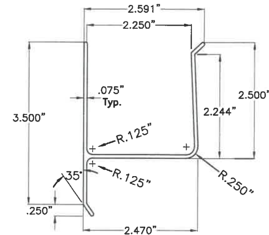
② REVERSED "h" TRACK
