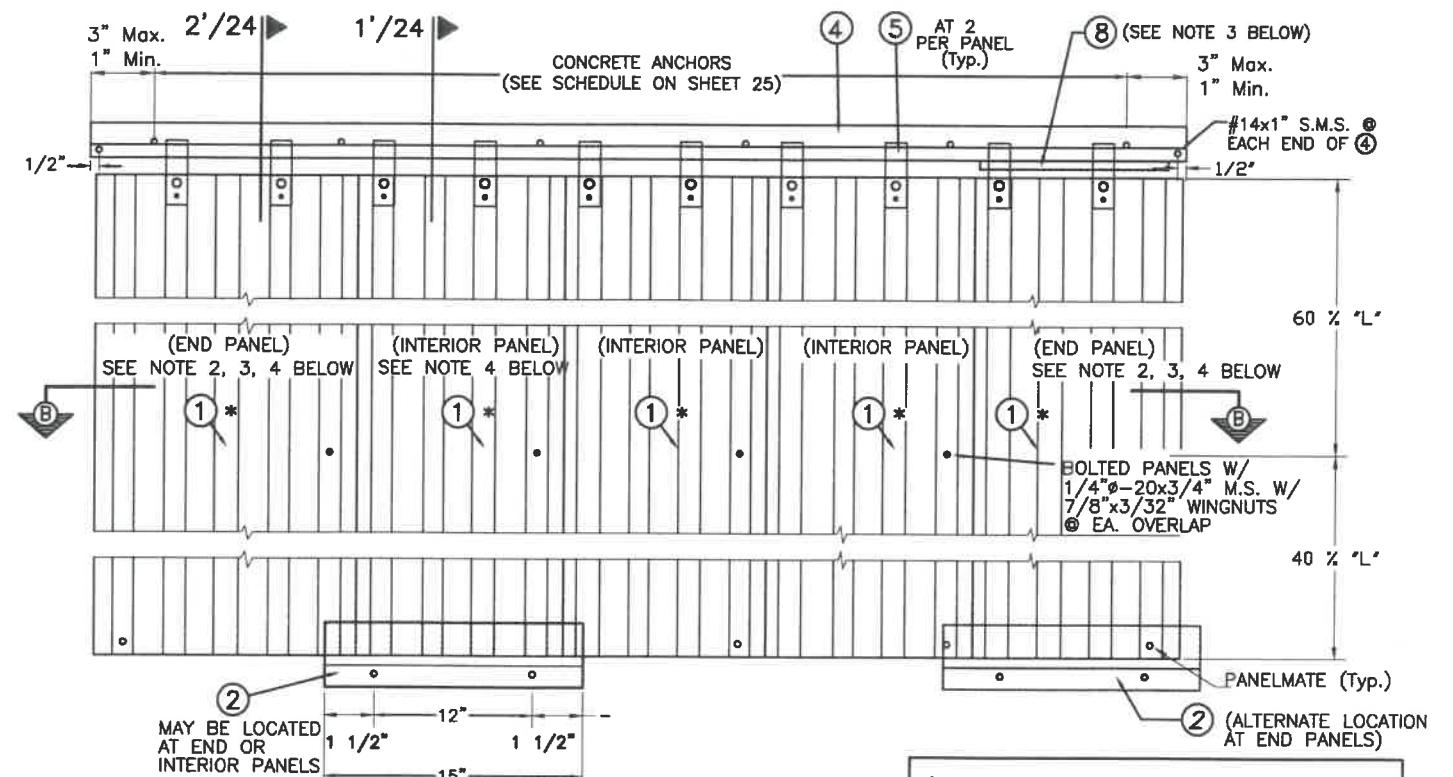
TYPICAL ELEVATION FOR SERIES 1000 E-Z HANG STORM PANEL ① SYSTEM
