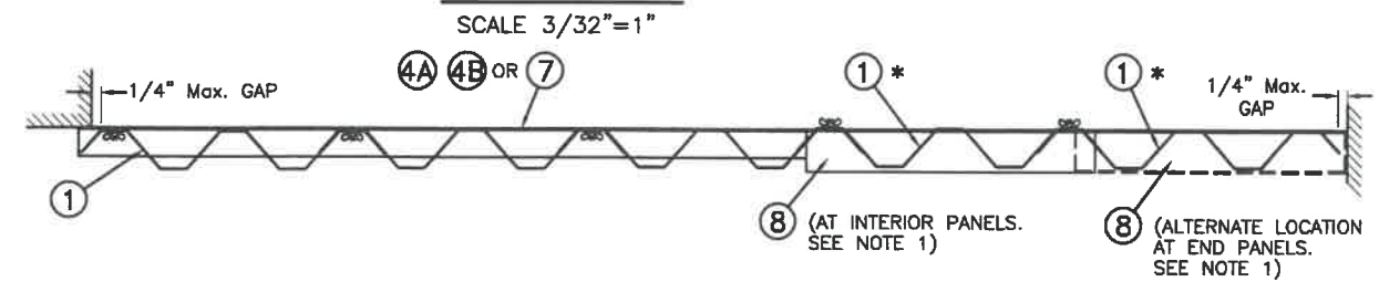
SECTION B-B SCALE 3/32"=1"
