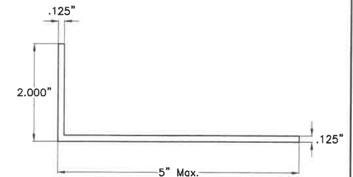
⑥ 2"x5" (Max.) ALUM. ANGLE
