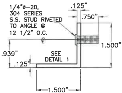
4B ANGLE WITH REVERSE STUD
