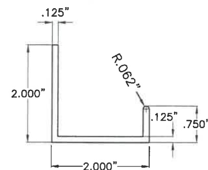
④ "J" TRACK
