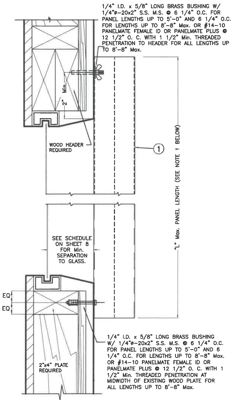
DIRECT MOUNTING INSTALLATION ALTERNATIVE 6W SCALE 3/8=1"
