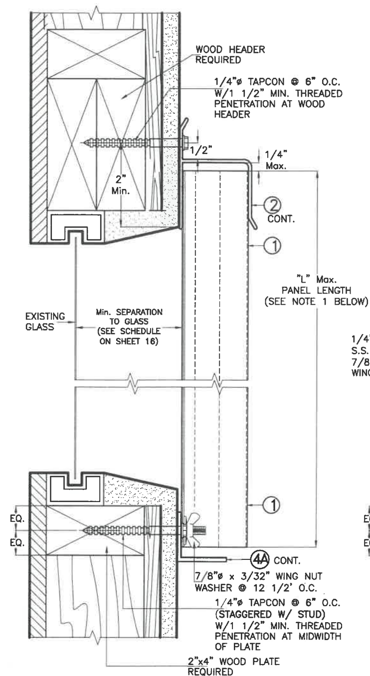
WALL MOUNTING INSTALLATION ALTERNATIVE 6AW ● REGULAR PANEL SCALE 3/8"=1"
