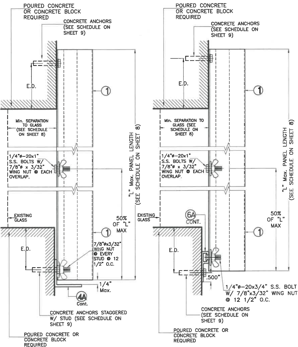
DIRECT AND WALL MOUNTING INSTALLATION SECTION 8 SCALE 3/8"=1"
