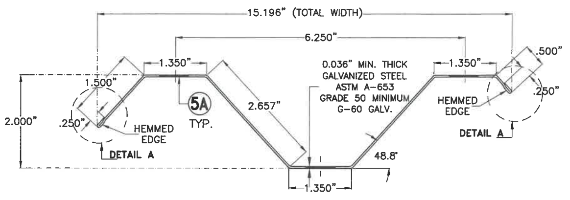
1A END STORM PANEL
