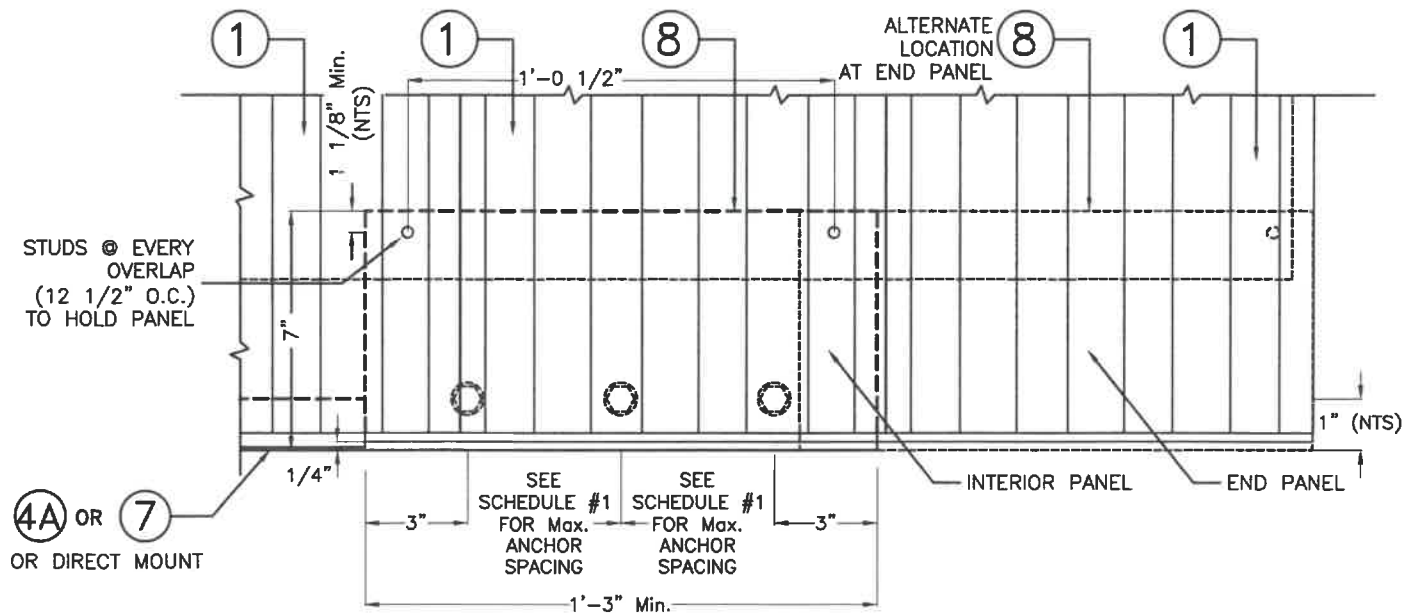
DETAIL 1 : WALL MOUNTING INSTALLATION (APPLICABLE TO SCHEDULE 1) SCALE: 3/16" = 1"
