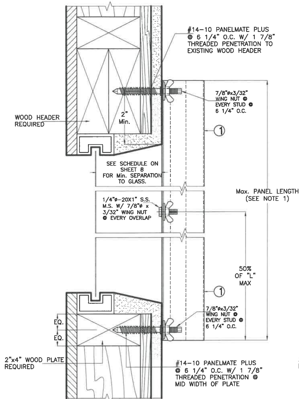
DIRECT MOUNTING INSTALLATION ALTERNATIVE 8W SCALE 3/8=1"
