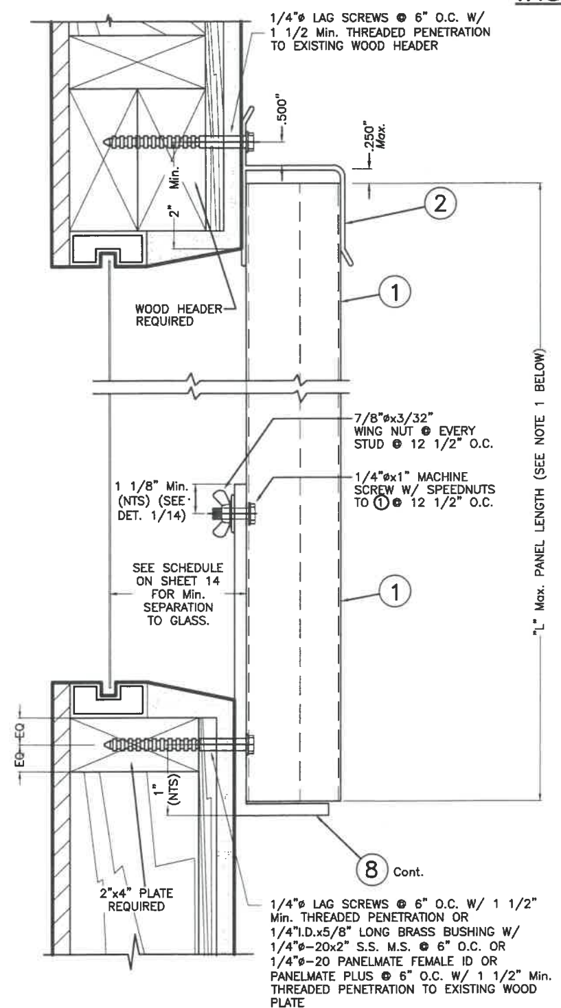
WALL MOUNTING INSTALLATION ALTERNATIVE 1W SCALE: 3/8" = 1"
