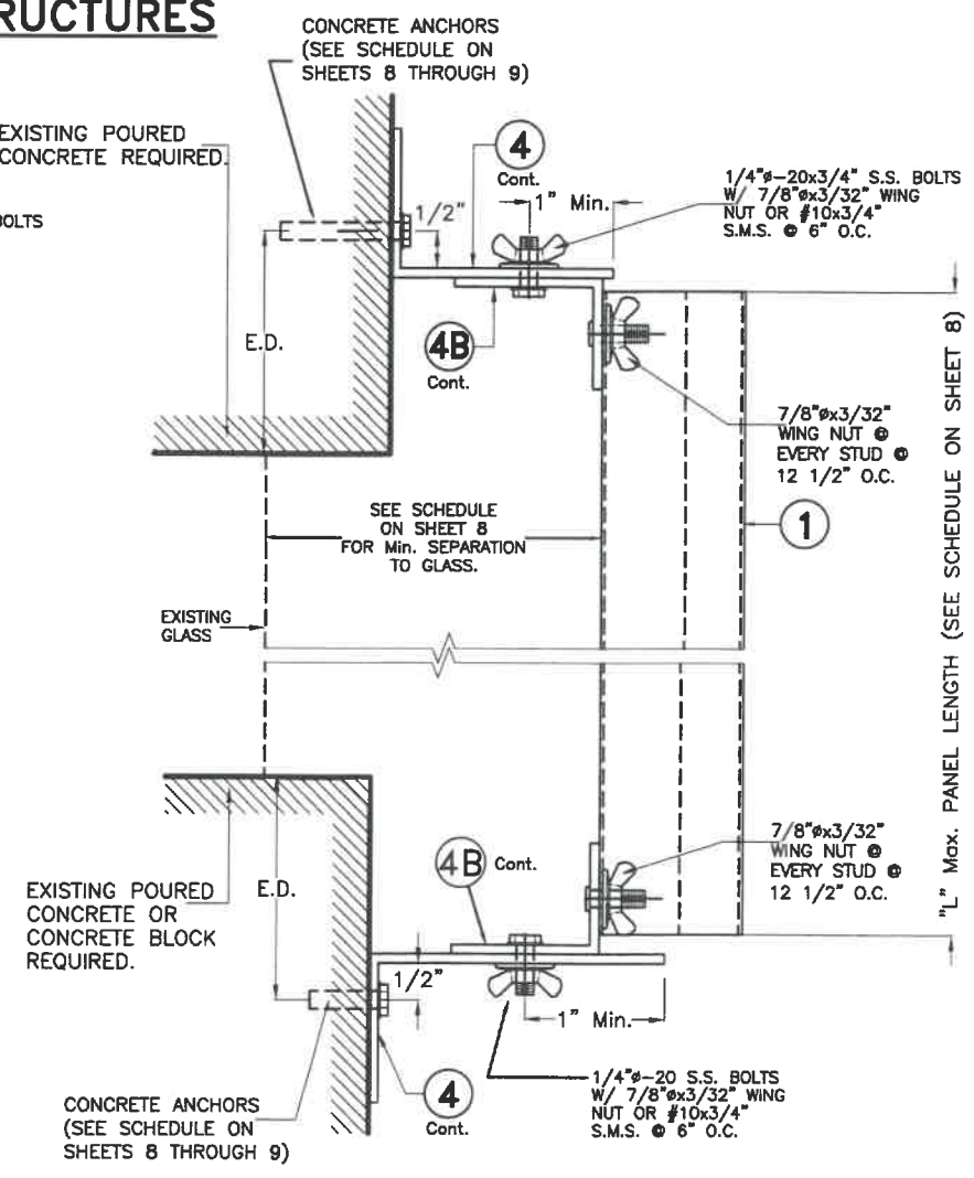
ALTERNATE BUILD OUT MOUNTING SECTION 4 SCALE 3/8=1"
