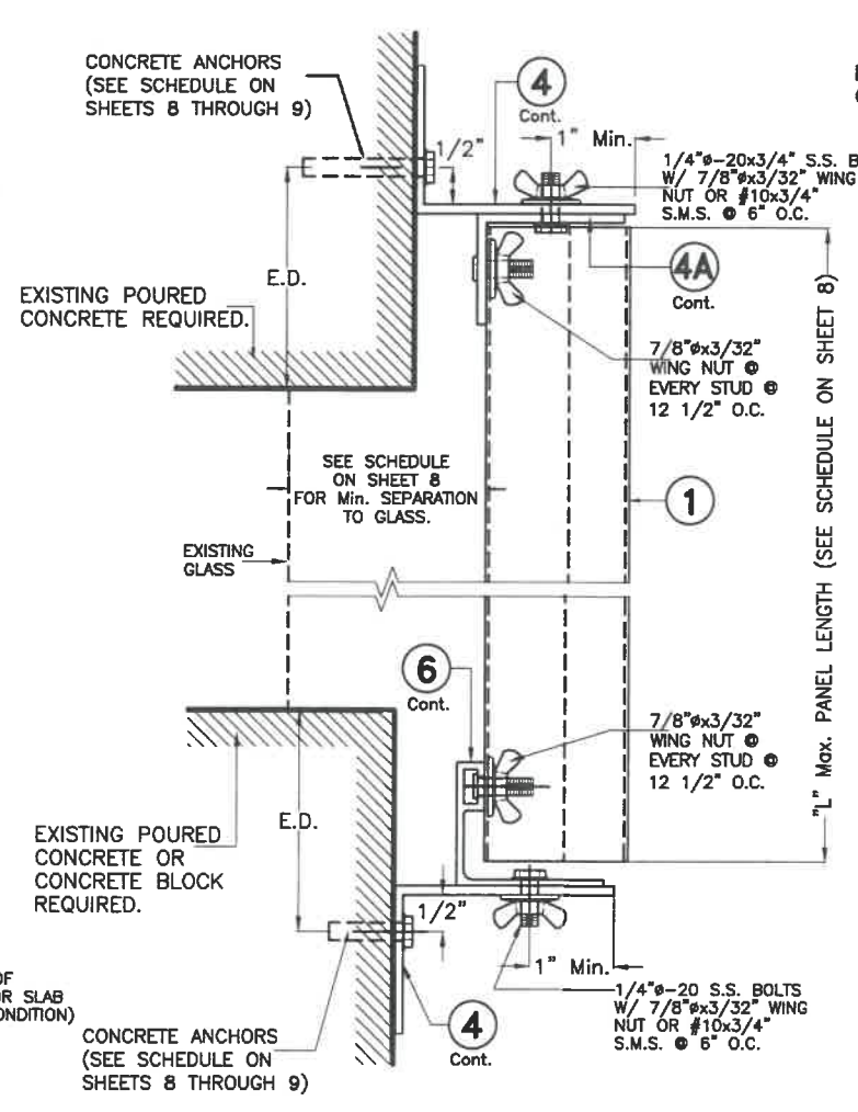
BUILD OUT MOUNTING SECTION 3 SCALE 3/8=1"
