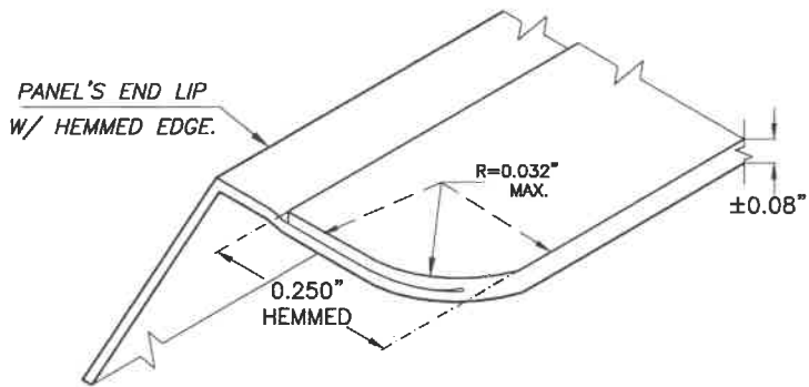
ISOMETRIC VIEW DETAIL A ROUNDED CORNER @ ENDS OF PANEL'S END LIP W/ HEMMED EDGE. (N.T.S)
