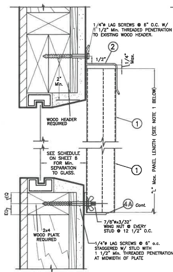
WALL MOUNTING INSTALLATION - ALTERNATIVE 2W SCALE: 1/4" = 1"
