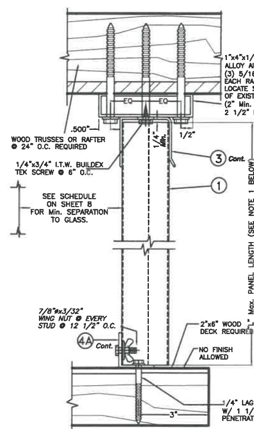
CEILING & FLOOR MOUNTING INSTALLATION - ALTERNATIVE 4W (SECTION AT TOP IS LIMITED TO +55.5-67.0 MAX. A.S.D. DESIGN PRESSURE RATING) SCALE: 1/4" = 1"
