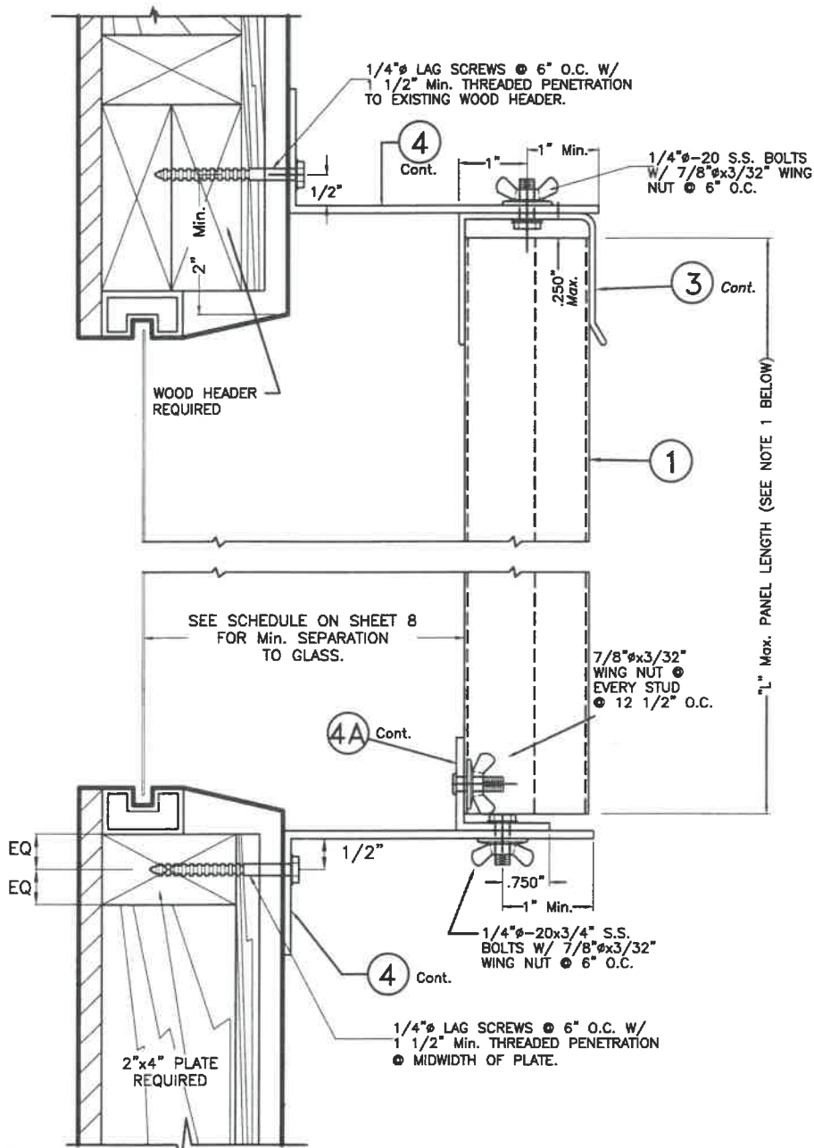
BUILD-OUT MOUNTING INSTALLATION ALTERNATIVE 7W SCALE 3/8=1"
