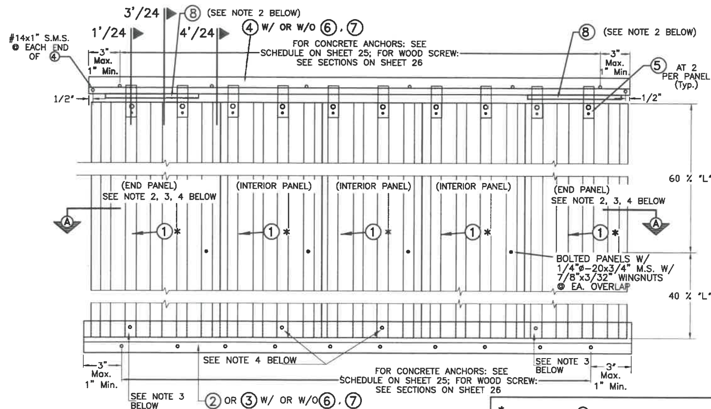
TYPICAL ELEVATION FOR SERIES 2000 E-Z HANG STORM PANEL ① SYSTEM
