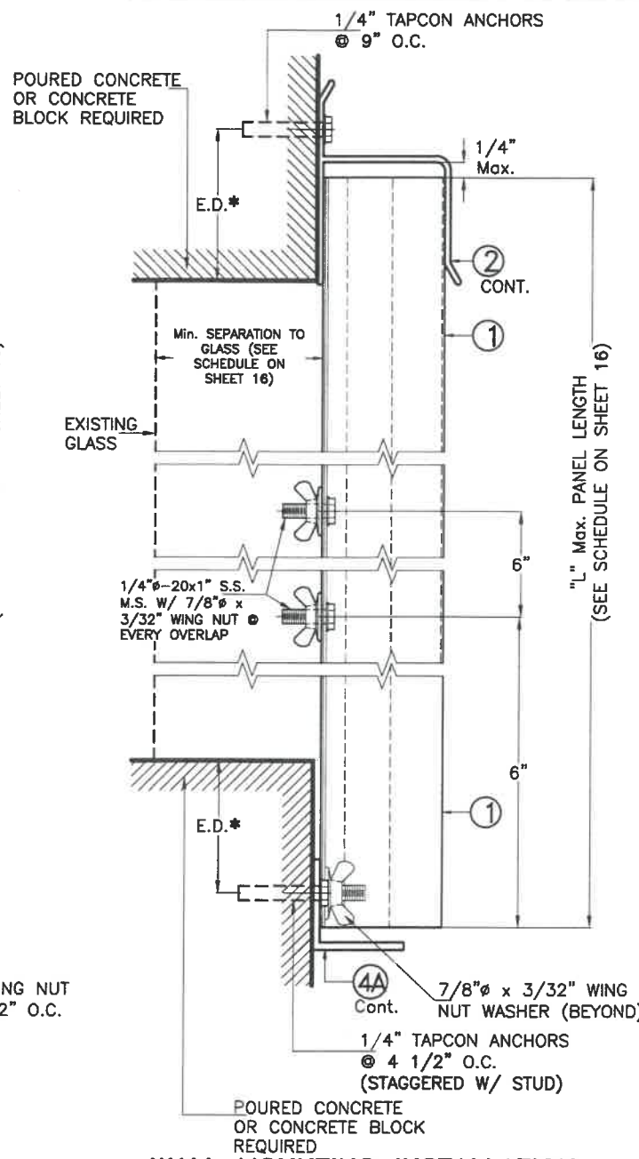
WALL MOUNTING INSTALLATION SECTION 3B ● LIFE SAFETY PANEL SCALE 3/8"=1"
