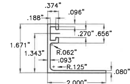
6 "F" TRACK ANGLE
